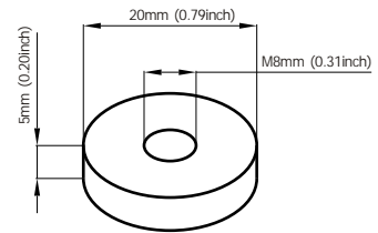
Terminal Dimensions
